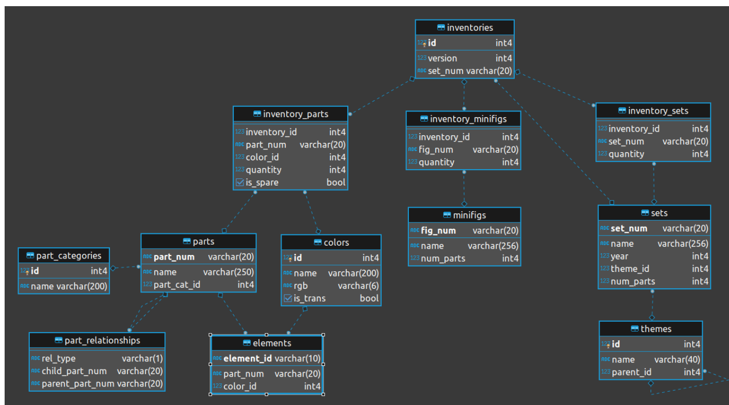
Schema Diagram for LEGO datafiles (click to expand)
